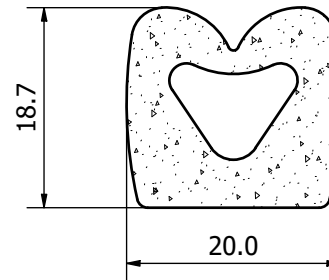
Front View ( 2 : 1 )
